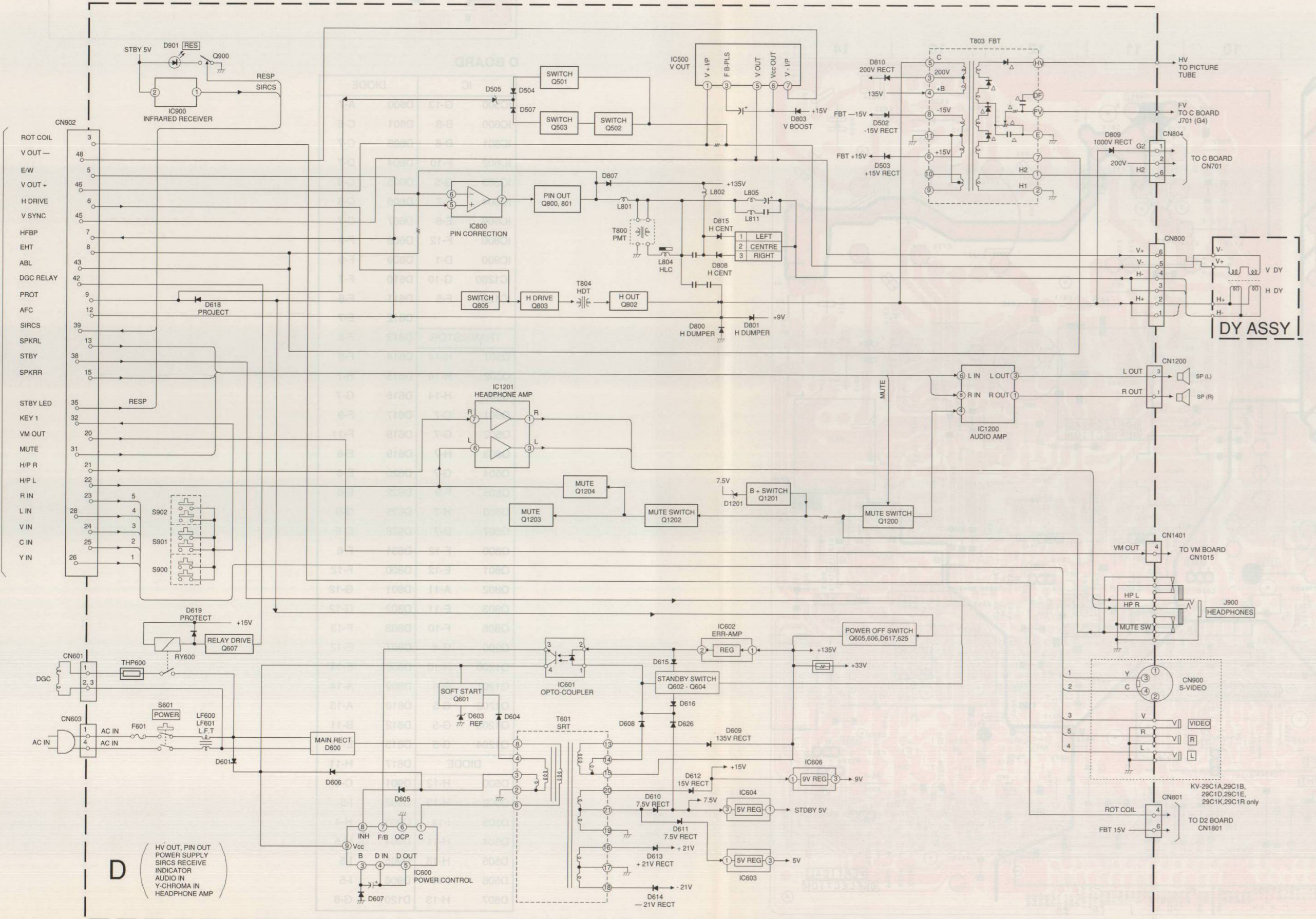
5-1. BLOCK DIAGRAM (1)
