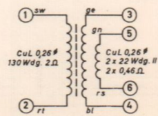
BV 9281-098 HF-Generatorspule HF Generator Coil Bobine oscillatrice HF
