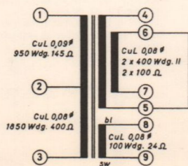
BV 9030-520 Treibertrafo Driver Transformer Transfo Driver
