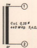
BV 9038-519 Drossel Choke Self
